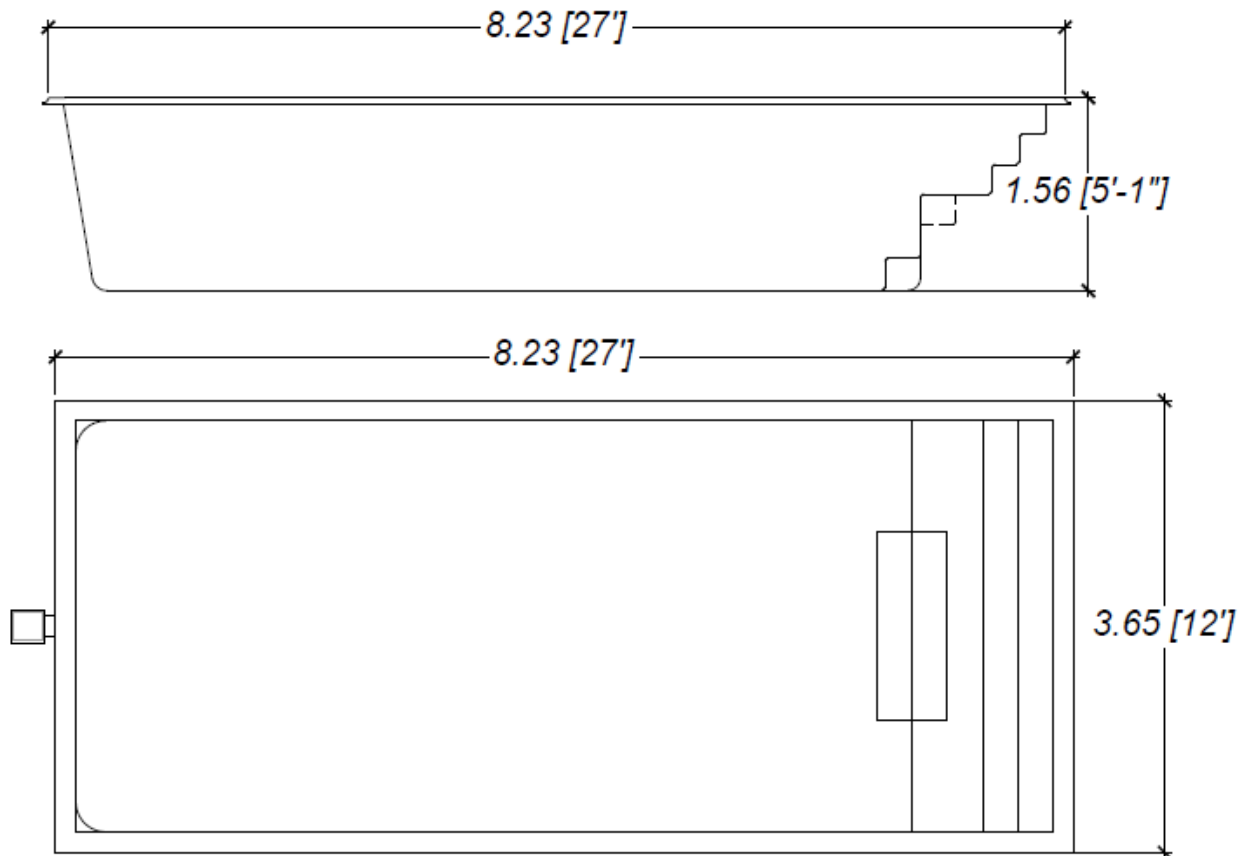
Structure of the swimming pool entirely in fiberglass.
