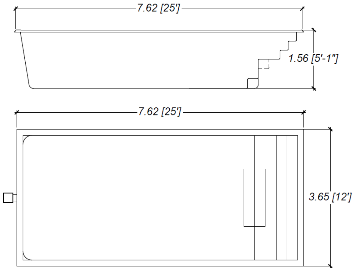
Structure of the swimming pool entirely in fiberglass.
