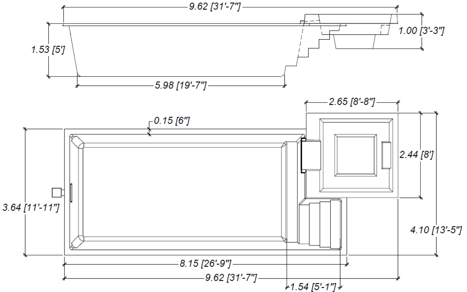
Structure of the swimming pool entirely in fiberglass.
