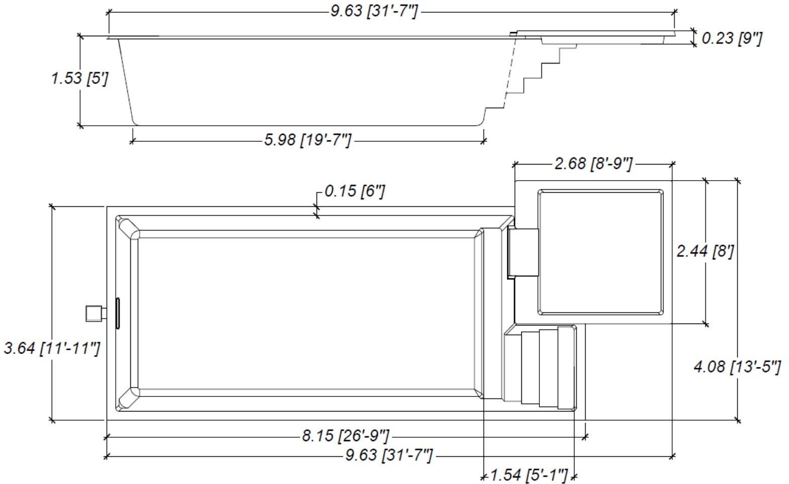
Structure of the swimming pool entirely in fiberglass.
